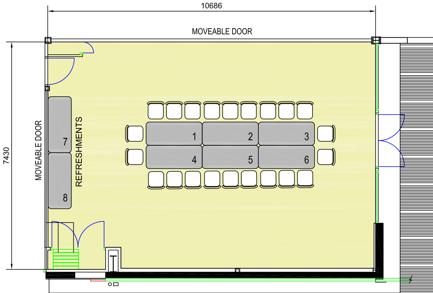
GARDEN ROOM 2
